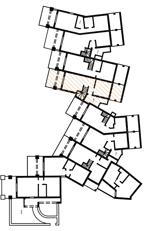
Piano terra
