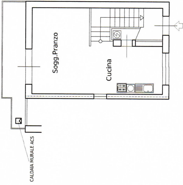
Piano Seminterrato h: mt 2,80
